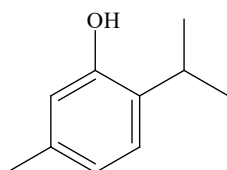
1. Carvacrol
